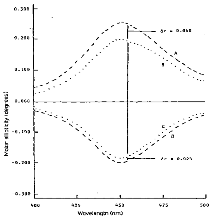
Fig. 5. Interaction of \Lambda -[Cr(en) 3 ] 3+ and \Delta -[Cr(en) 3 ] 3+ with R(+)-tartaric acid. (A) (+)- D [Cr(en) 3 ] 3+ circular dichroism spectrum; (B) circular dichroism spectrum of (+)- D [Cr(en) 3 ] 3+ with excess R(+)- D -tartaric acid; (C) circular dichroism spectrum of (-)- D [Cr(en) 3 ] 3+ with excess R(+)- D -tartaric acid; (D) circular dichroism spectrum of (-)- D [Cr(en) 3 ] 3+ .
