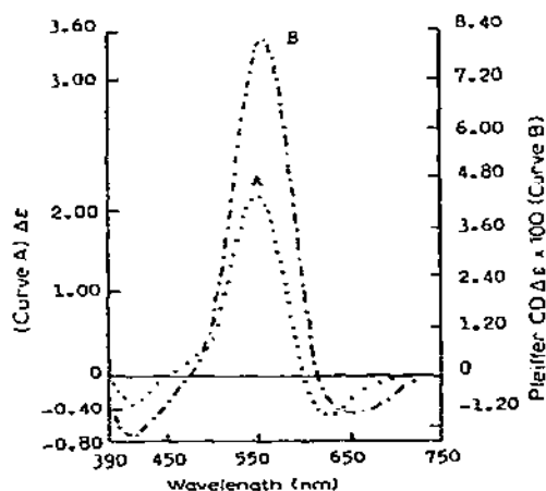
Fig. 1. (A) Circular dichroism spectrum of (+)\text{-D}[\text{Cr}(\text{ox})_3]^{3-} in \text{H}_2\text{O} . (B) Pfeiffer circular dichroism spectrum of \text{D,L-}[\text{Cr}(\text{ox})_3]^{3-} in water containing d -cinchonine hydrochloride (all measurements at 23^\circ\text{C} ).
